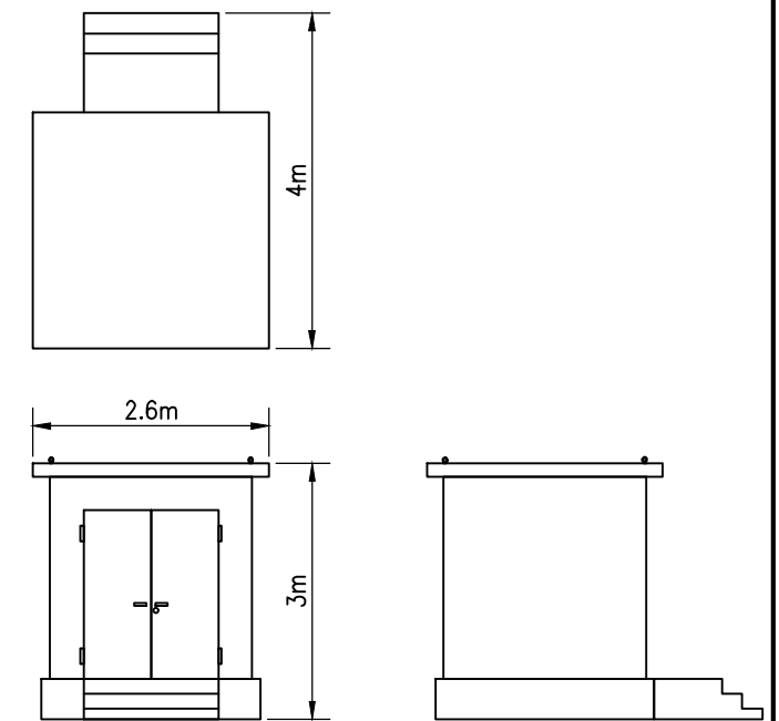
TYPICAL EXTERNAL TRANSFORMER ELEVATIONS
